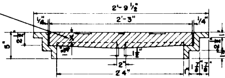
SECTION - MANHOLE AND FRAME
