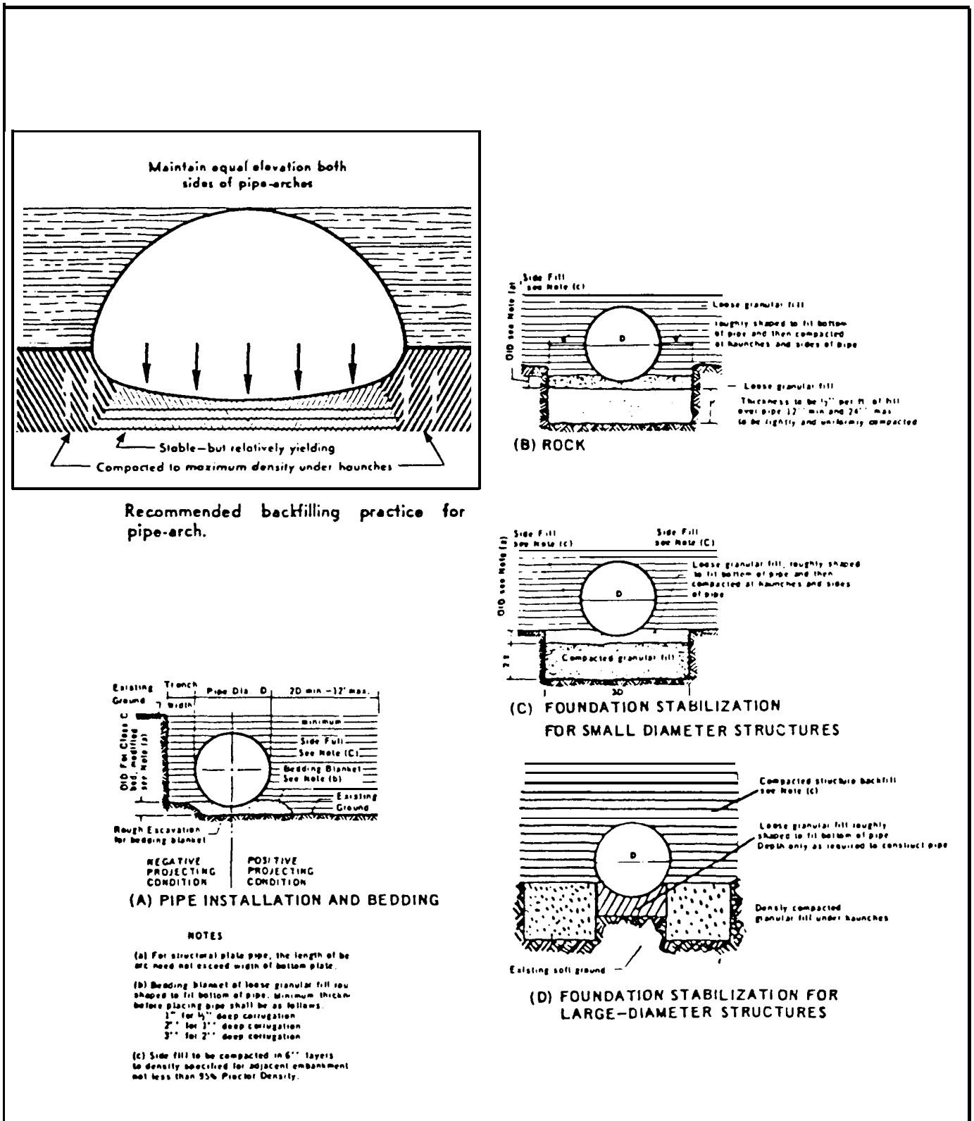
Figure C-5. Flexible Pipe Bedding and Installation
