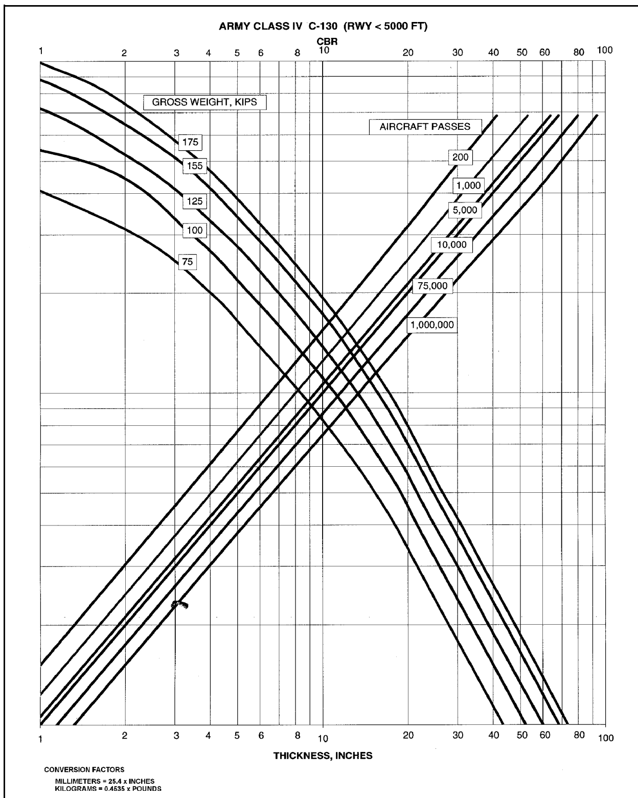
Figure 10-5. Flexible pavement design curves for Army Class IV airfields (C-130 aircraft) with runway \leq 1,525 meters ( \leq 5,000 feet), types B and C traffic areas
