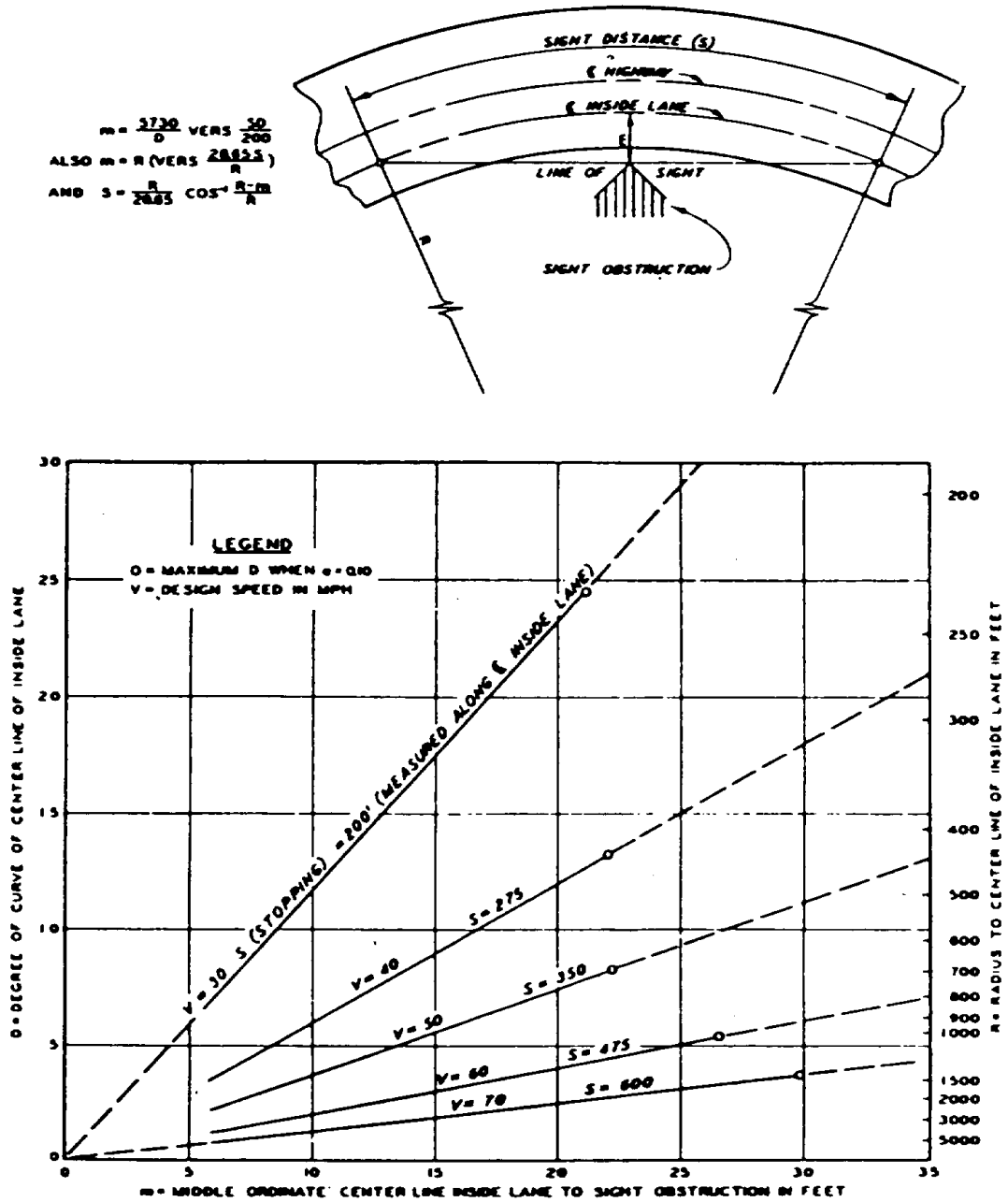
Figure 3-4. Stopping sight distance on horizontal curves and open road conditions.
